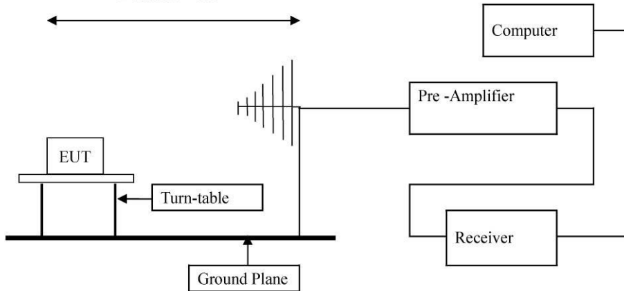
Block diagram of Test setup
